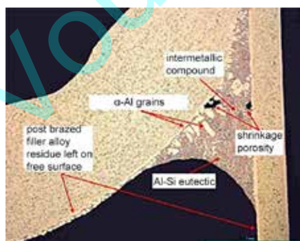
Fig. 2 • Metallographic structure of a tube to header joint – etched with hydrofluoric acid (HF).
