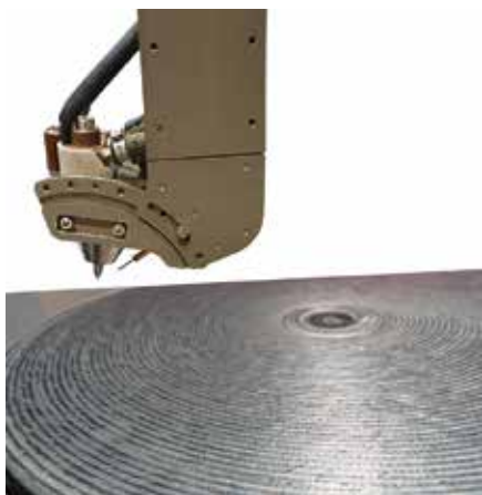
Fig. 5 • Adjustment of electrodes and wire for the cladding of the flange surface and example of a clad specimen.
