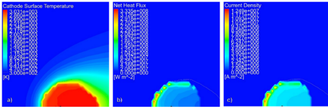
Fig. 2 • Temperature field (a), heat flux density (b) and electric current density of the molten pool (c), after [12].
