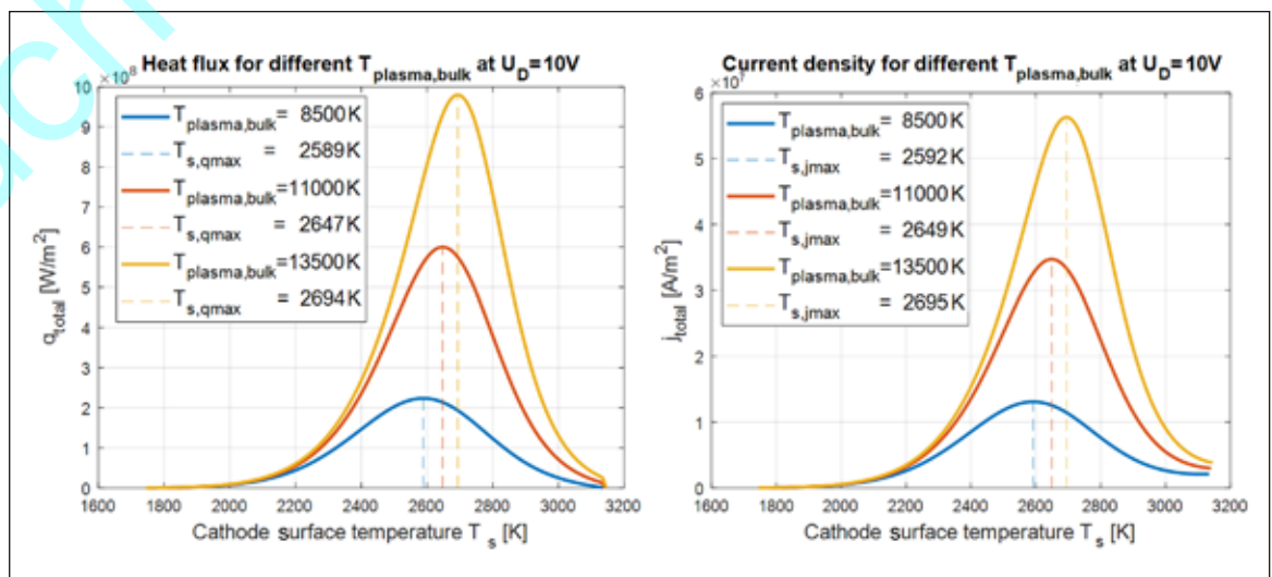
Fig. 1 • Heat flux density and electric current density according to the model from [12].
