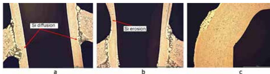
Fig. 3 • Examples of structural brazing phenomena; a) silicon diffusion, b) erosion, c) liquid film migration.
