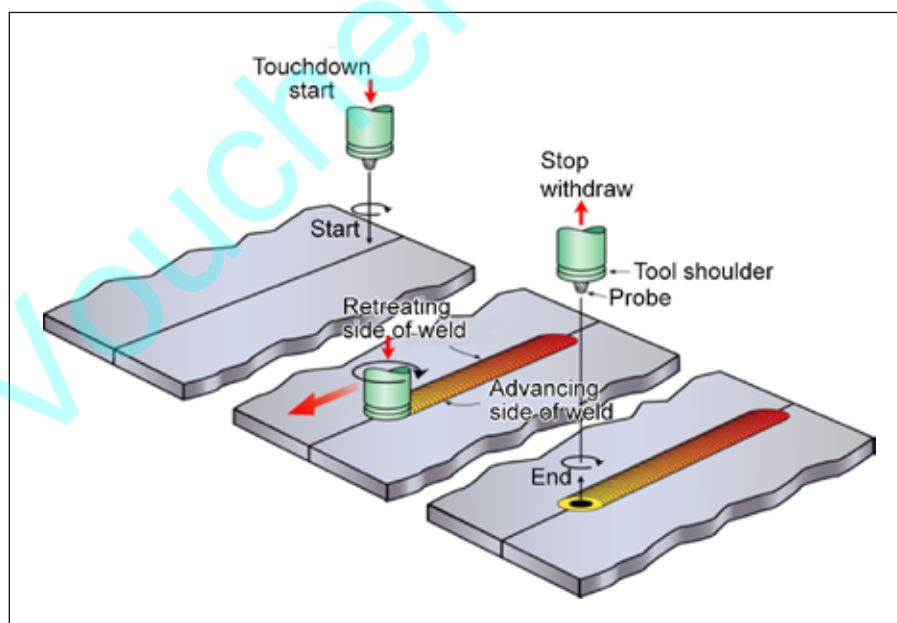
Fig. 1 • The basic principle of friction stir welding.
