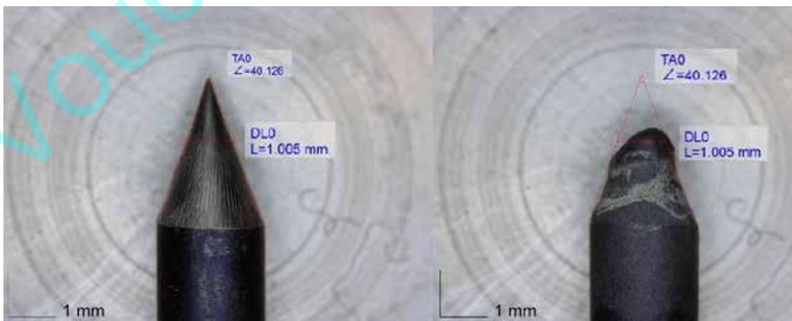
A ground electrode before welding (left) and after AC welding (right) with correct settings on the welding machine (Diameter Ø 2,4 mm, grinding angle 20° = tip angle 40°). Where did the tip go?
