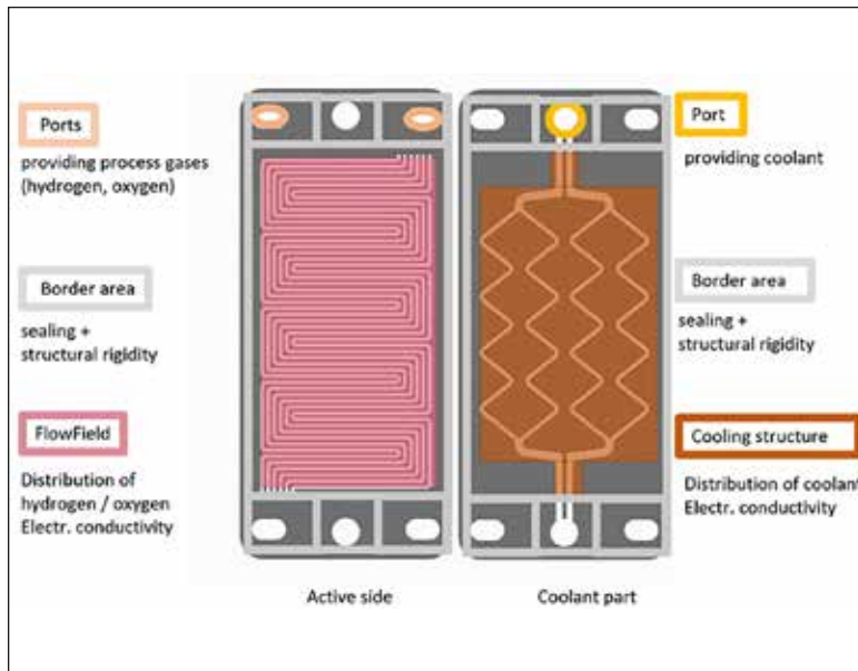
Fig. 2 • Locally resolved functional requirements for the bonding points on the active or cooling side of a bipolar panel. (Source: ZBT GmbH)
