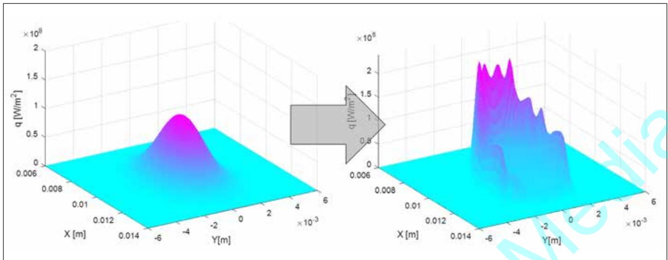
Fig. 3 • Comparison between the conventional (Gaussian) notion of heat flux density (left) and the distribution of heat flux density considering a physics-based cathode model [12].
