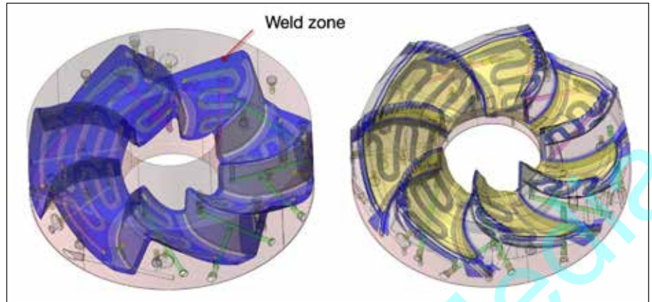
Design of the prepress part (left) and the tool insert (right) (Picture: FKT)
