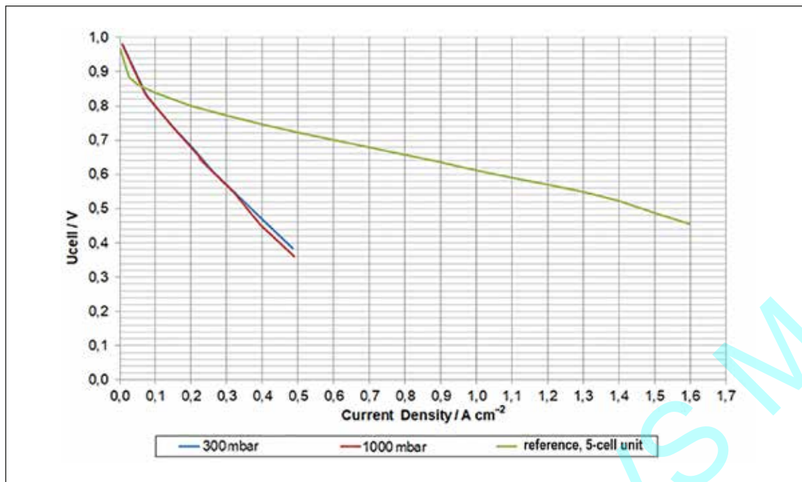
Fig. 7 • Voltage – current density curves of a foil-based edge plate operated in the test rig. (Source: ZBT GmbH)
