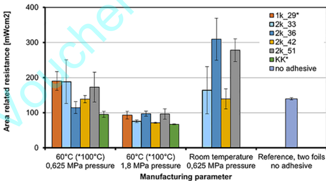
Fig. 4 • Area-specific volume resistances of bonded sandwich specimen and one reference. (Source: ZBT GmbH)
