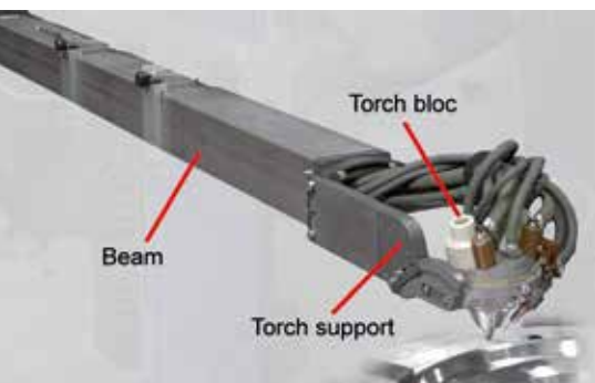
Fig. 2 • Reclining welding lance for the TIG er process.
