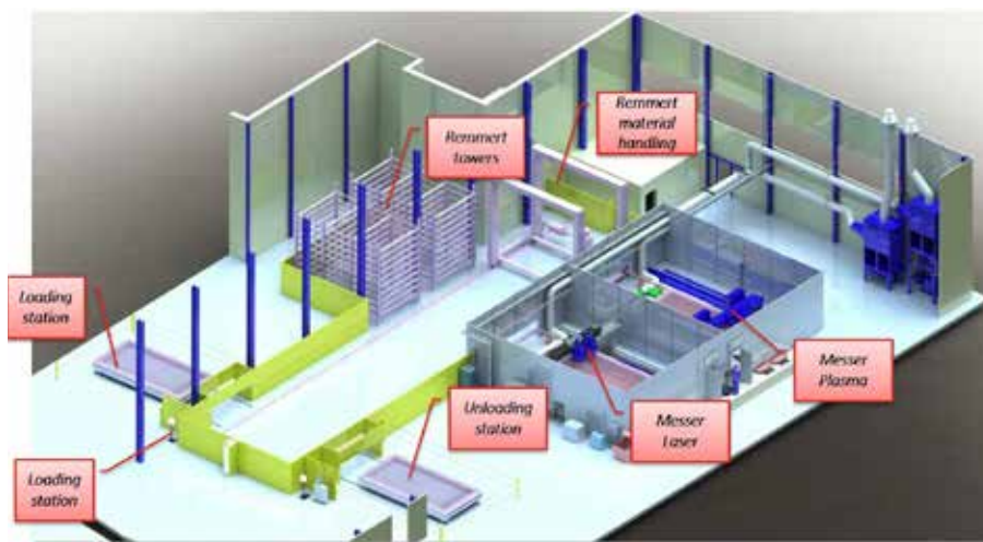
Overview of the automation system in the production hall with Messer machines and Remmert material handling system. (All photos: Messer Cutting Systems)
