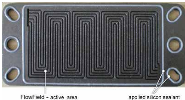
Fig. 5 • Flow field sealed with silicone. (Source: ZBT GmbH)
