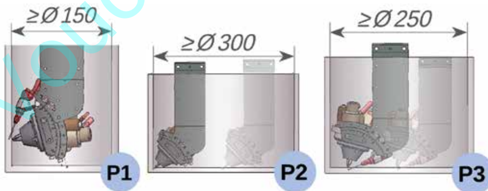
Fig. 3 • Preferred positions P1, P2 and P3: position P1 has to be taken if a cylindrical body has to be cladded at the inside; position P2 is chosen if the wire impact shall be suitable for cladding of a corner; position P3 is selected if the bottom of a workpiece shall be cladded (left). Example of a workpiece where the three preferred torch positions are used (right).
