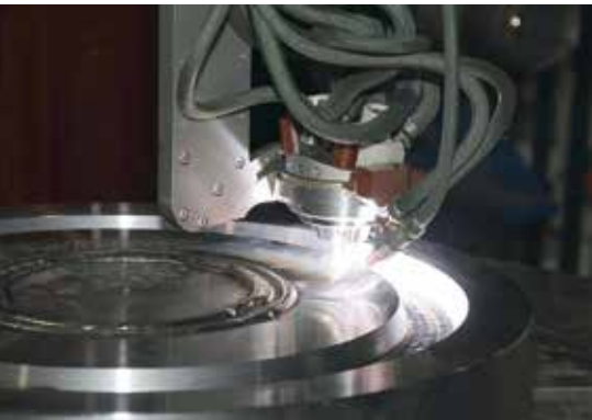
Fig. 1 • TIG welding overlay cladding with reclining lance.
