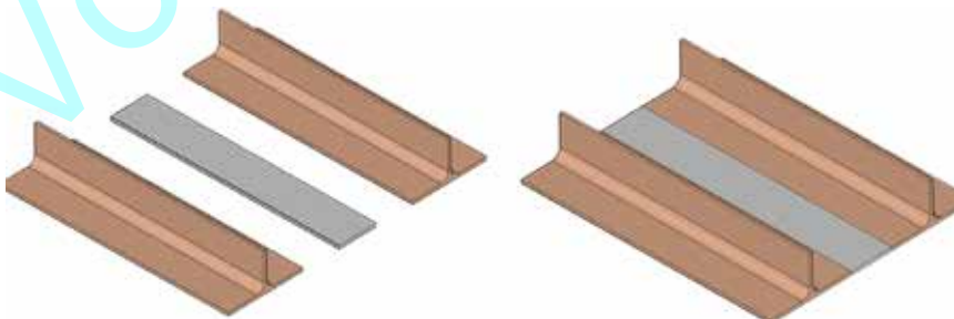
Fig. 5 • Concept of stiffened panel construction from rolled T sections spaced apart with rolled plate (left); integrally stiffened plate demonstration piece fabricated by friction stir butt welding two rolled T sections to a steel plate.
