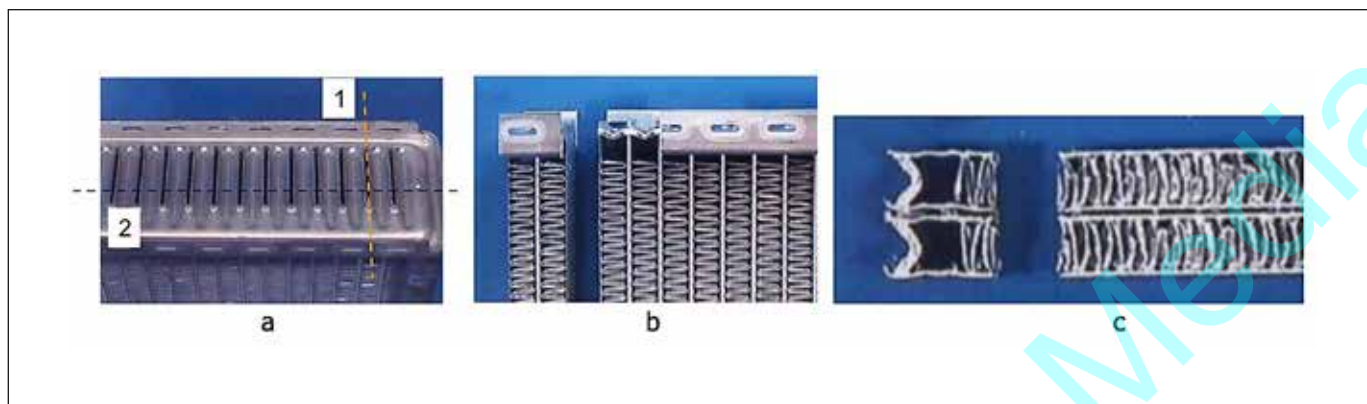
Fig. 1 • Cutting of a radiator for examination of the joint quality; a) brazed part with marked cutting lines, b) part after cutting along line 1, c) part after cutting along line 2.
