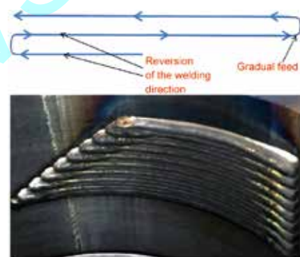
Fig. 8 • Clad surface obtained by the "Patch" mode including reversion and welding speed correction.
