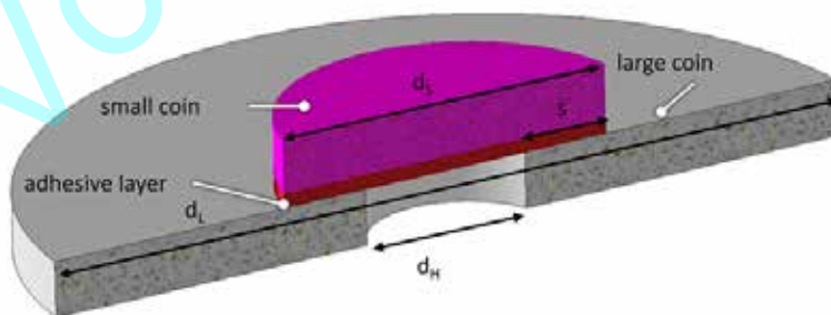
Fig. 3 • Sectional view of a coin specimen for measuring hydrogen tightness. (Source: ifs TU Braunschweig)
